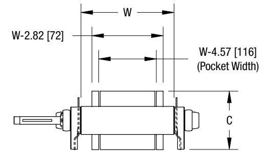
Sidewall Cleated Belt
