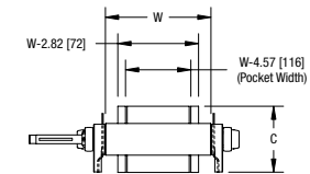
Sidewall Cleated Belt
