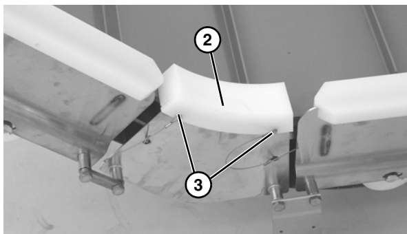
Figure 18 (Lower Knuckle)
