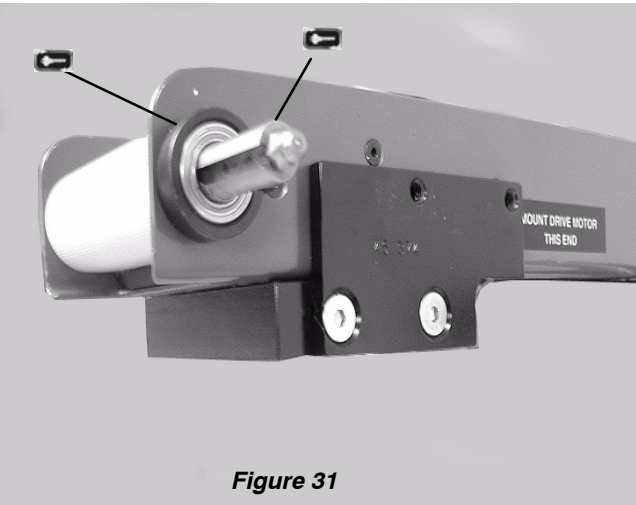
Mounting Package attached to a 4100 series conveyor.
