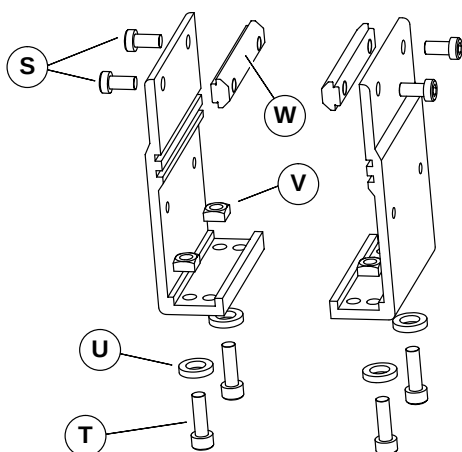
Mounting Brackets for Flat Belt Conveyor Figure 8
