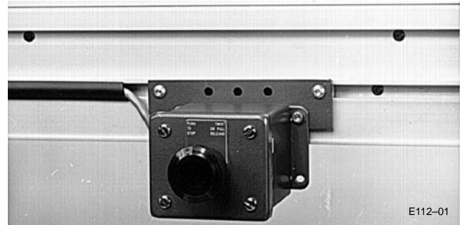
Figure 1: Illuminated E-Stop Kit Installed (75-40)
