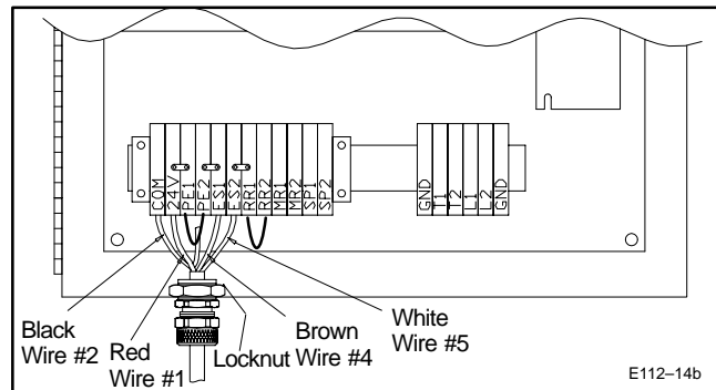
Figure 14: Sample E-Stop to impac Wiring Connections
