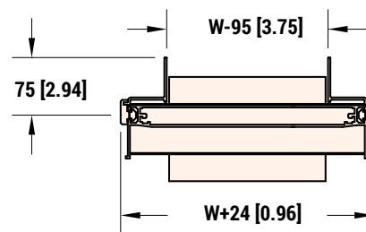
Cleated LPZ Profile 3 64 mm (2.5 in) Aluminum Side
