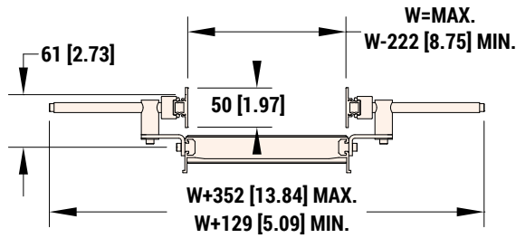
Profile 39 Horizontal Adjustable Guiding 50 mm (2 in) HDPE Face
