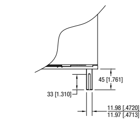
2200 Belted & Modular Belt End Drive:
