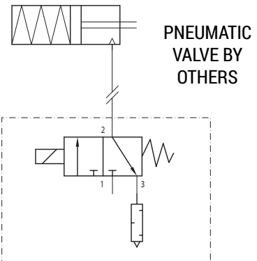
PNEUMATIC SCHEMATIC
