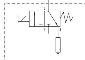
PNEUMATIC SCHEMATIC
