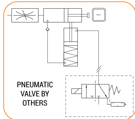
PNEUMATIC SCHEMATIC
