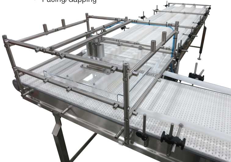
90 Degree Transfer with Product Stager
