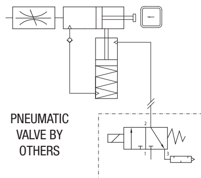
PNEUMATIC SCHEMATIC
