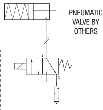
PNEUMATIC SCHEMATIC
