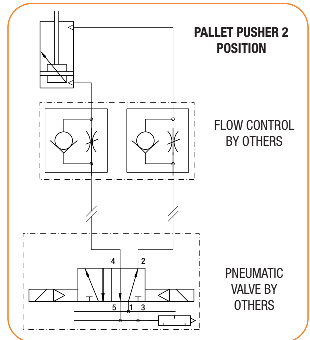
PNEUMATIC SCHEMATICS
