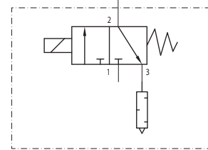
PNEUMATIC SCHEMATIC
