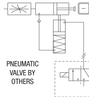
PNEUMATIC SCHEMATIC
