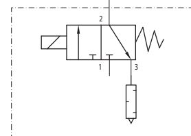
PNEUMATIC SCHEMATIC
