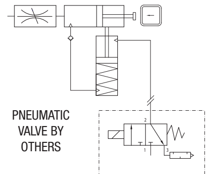
PNEUMATIC SCHEMATIC
