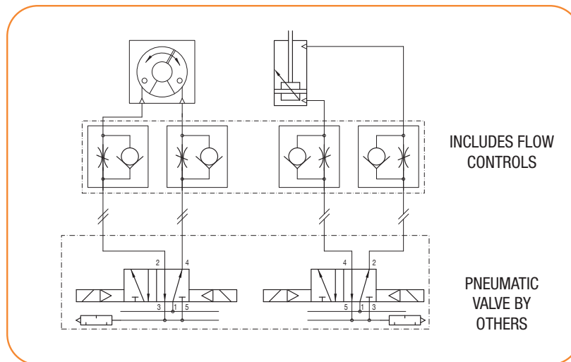
PNEUMATIC SCHEMATIC
