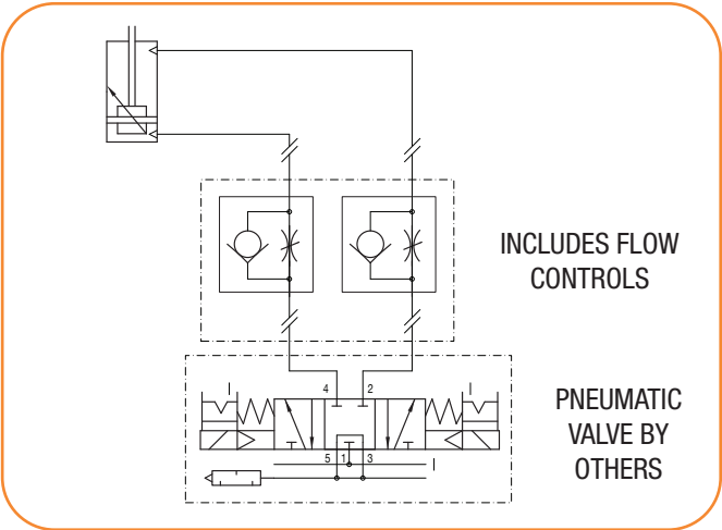
PNEUMATIC SCHEMATIC
