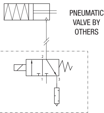
PNEUMATIC SCHEMATIC
