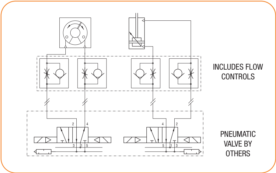
PNEUMATIC SCHEMATIC
