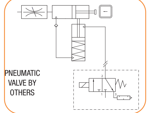
PNEUMATIC SCHEMATIC
