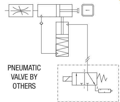
PNEUMATIC SCHEMATIC
