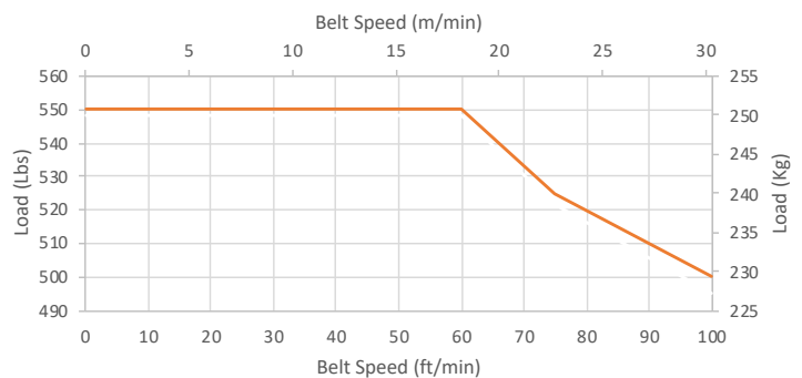
Maximum Accumulated Load - Non-cushioned Pallet Stop
