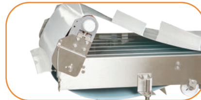
STANDARD FEATURE: Tip-Up Tail**
