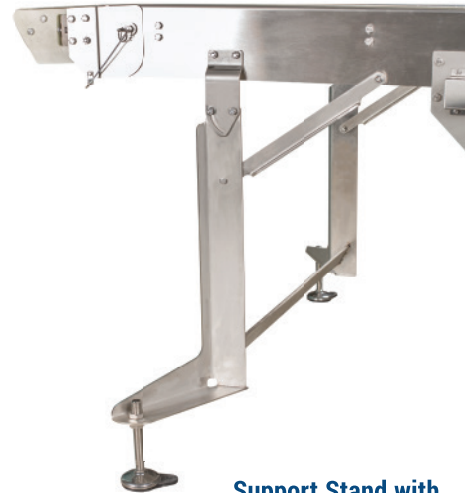
Support Stand with optional outrigger and diagonal brace shown
