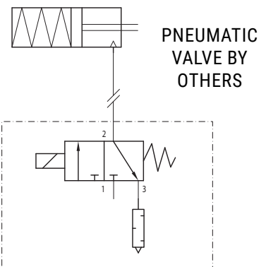
PNEUMATIC SCHEMATIC
