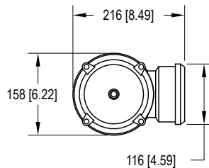
Chart 10 90° eDrive NEMA C-Face VFD Rated
