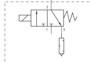
PNEUMATIC SCHEMATIC
