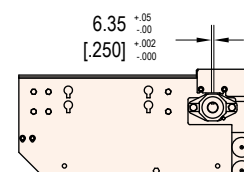
Side Motor Mount
