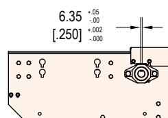
Bottom Motor Mount
