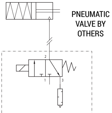
PNEUMATIC SCHEMATIC
