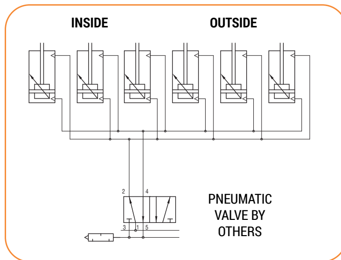
PNEUMATIC SCHEMATIC
