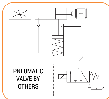
PNEUMATIC SCHEMATIC
