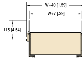
-04 76 mm (3 in) Aluminum High Side
