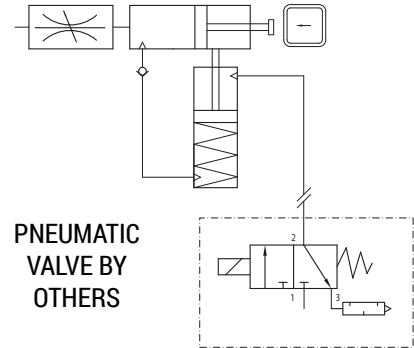
PNEUMATIC SCHEMATIC
