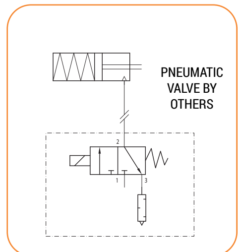
PNEUMATIC SCHEMATIC
