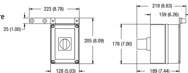
Manual Motor Starter
