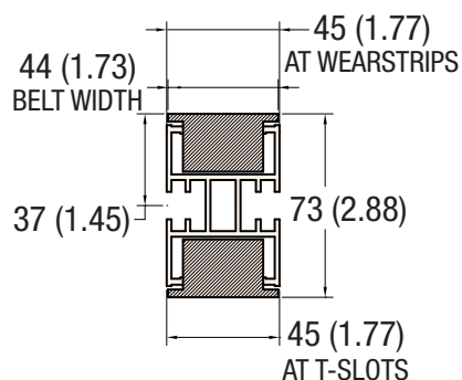
45 MM WIDTH
