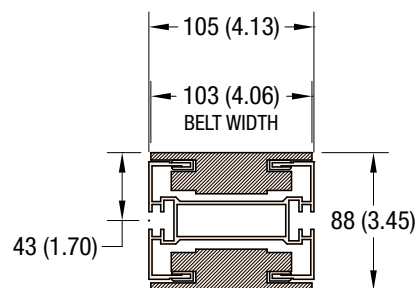
105 MM WIDTH
