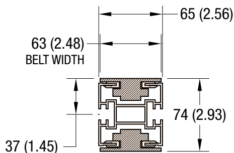
65 MM WIDTH
