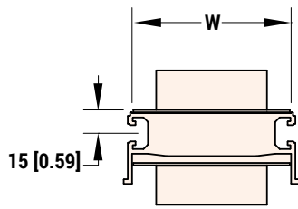
Cleated Profile 0 Low Side Cleated
