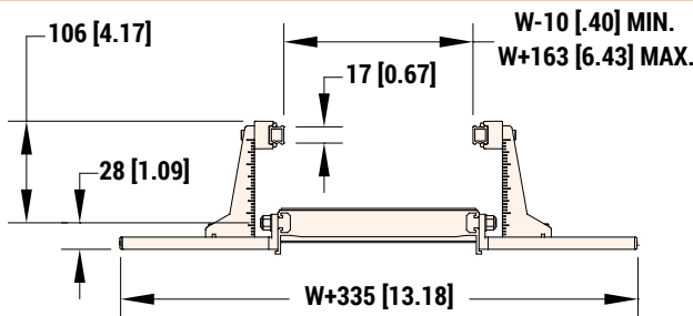
Profile 46 Outboard Adjustable Guiding Aluminum Face
