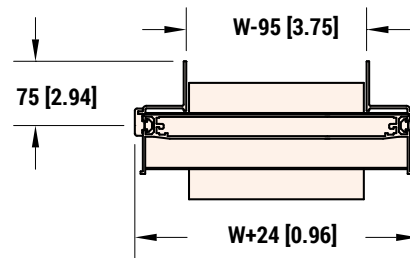
Cleated LPZ Profile 3 64 mm (2.5 in) Aluminum Side
