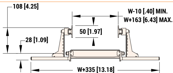
Profile 36 Outboard Adjustable Guiding 50 mm (2 in) HDPE Face
