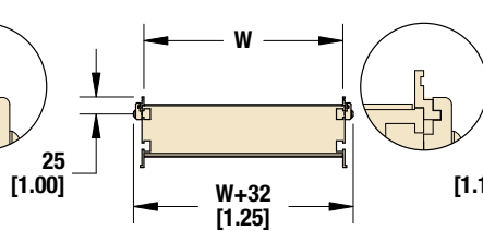
13 (0.5 in) Aluminum Side (Not available on Precision Move)
