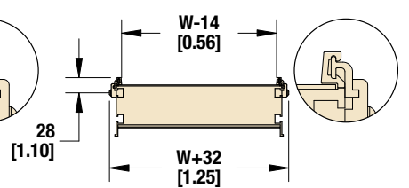
13 (0.5 in) Extruded Plastic (Do not use with belt #64) (Not available on Precision Move)
