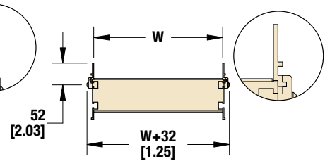
38 mm (1.5 in) Aluminum Side
