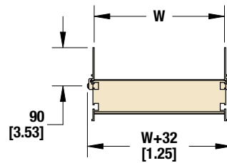
76 mm (3 in) Aluminum Side
