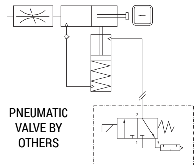
PNEUMATIC SCHEMATIC
