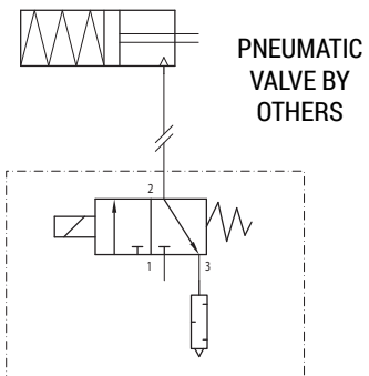
PNEUMATIC SCHEMATIC
