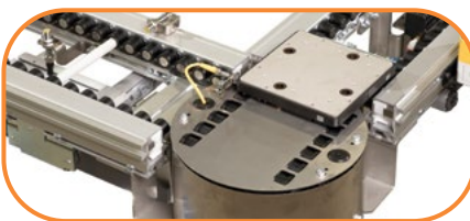
Turn & Transfer
