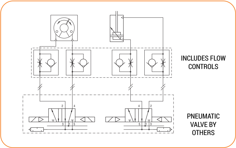
PNEUMATIC SCHEMATIC
