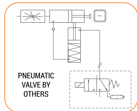
PNEUMATIC SCHEMATIC
