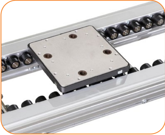
Driven Rollers
