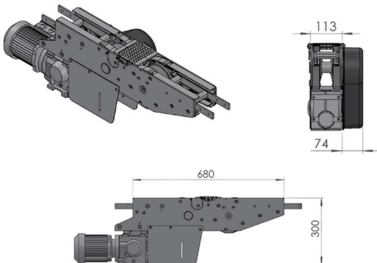
FC Combined Suspended Drive & Idler (LEFT)
