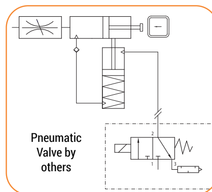
Cushioned Pneumatic Schematic
