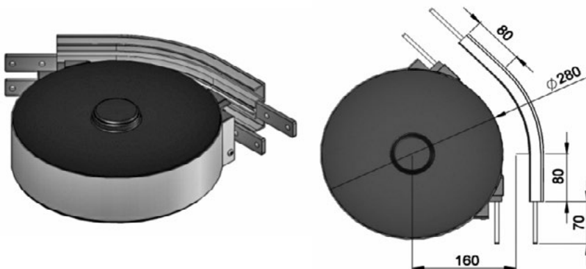
FM Wheel Bend 30°
