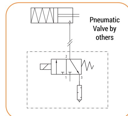
Non-Cushioned Pneumatic Schematic
