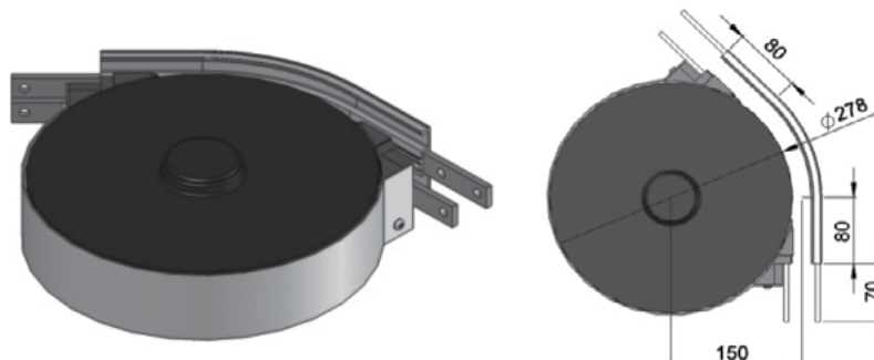
FK Wheel Bend 45°
